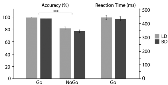
Fig. 1. Accuracy and reaction times (means \pm standard errors) are shown for the low drinking (LD) and binge drinking (BD) groups and for the Go and NoGo conditions.
