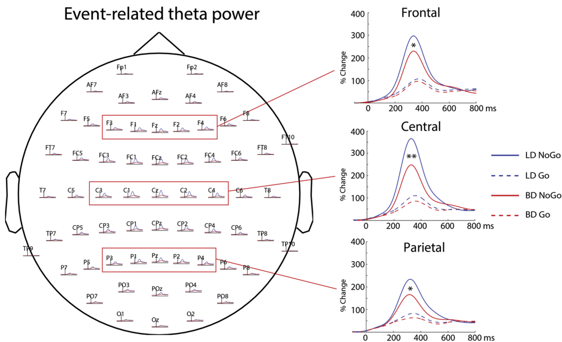
Fig. 2. Frontal, central, and parietal electrode clusters and group average time courses for event-related theta power averaged within each cluster. Overall, event-related theta power was greater on NoGo trials, it peaked at ~350 ms, and it was most prominent in the central region. BD participants had reduced NoGo theta power in all three regions compared to LDs. * p < .05 , ** p < .01 .
