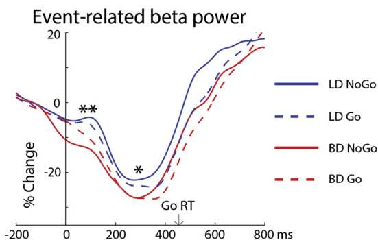
Fig. 3. Event-related beta power time course averaged over the central electrode cluster. LD participants show an early, transient increase in beta power (50–125 ms). * p < .05 , ** p < .01 . Average Go reaction time is marked by arrow.
